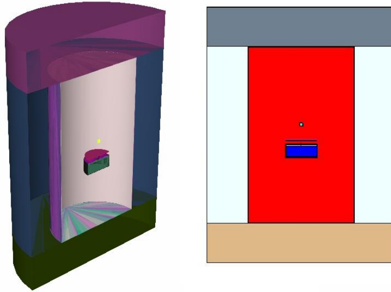
Figure 2. Sectional views of the planar detector within its shield with the tin-cadmium filter in place.
