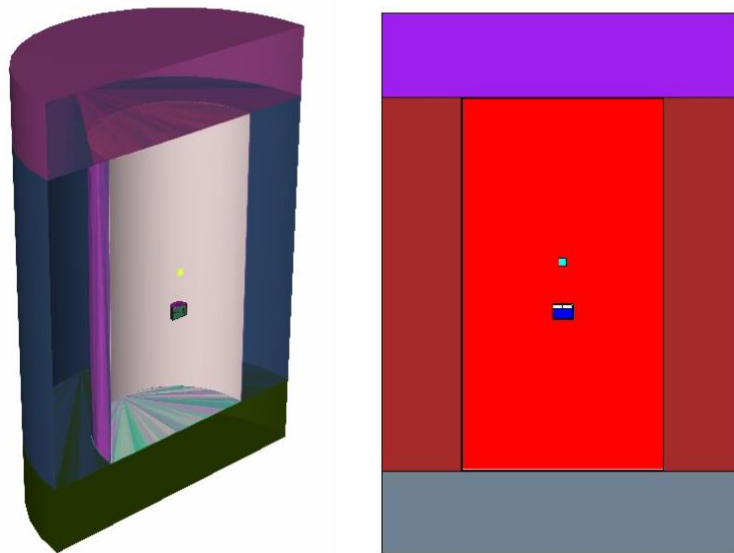
Figure 3. Sectional views of the LEGe detector within its shield.
