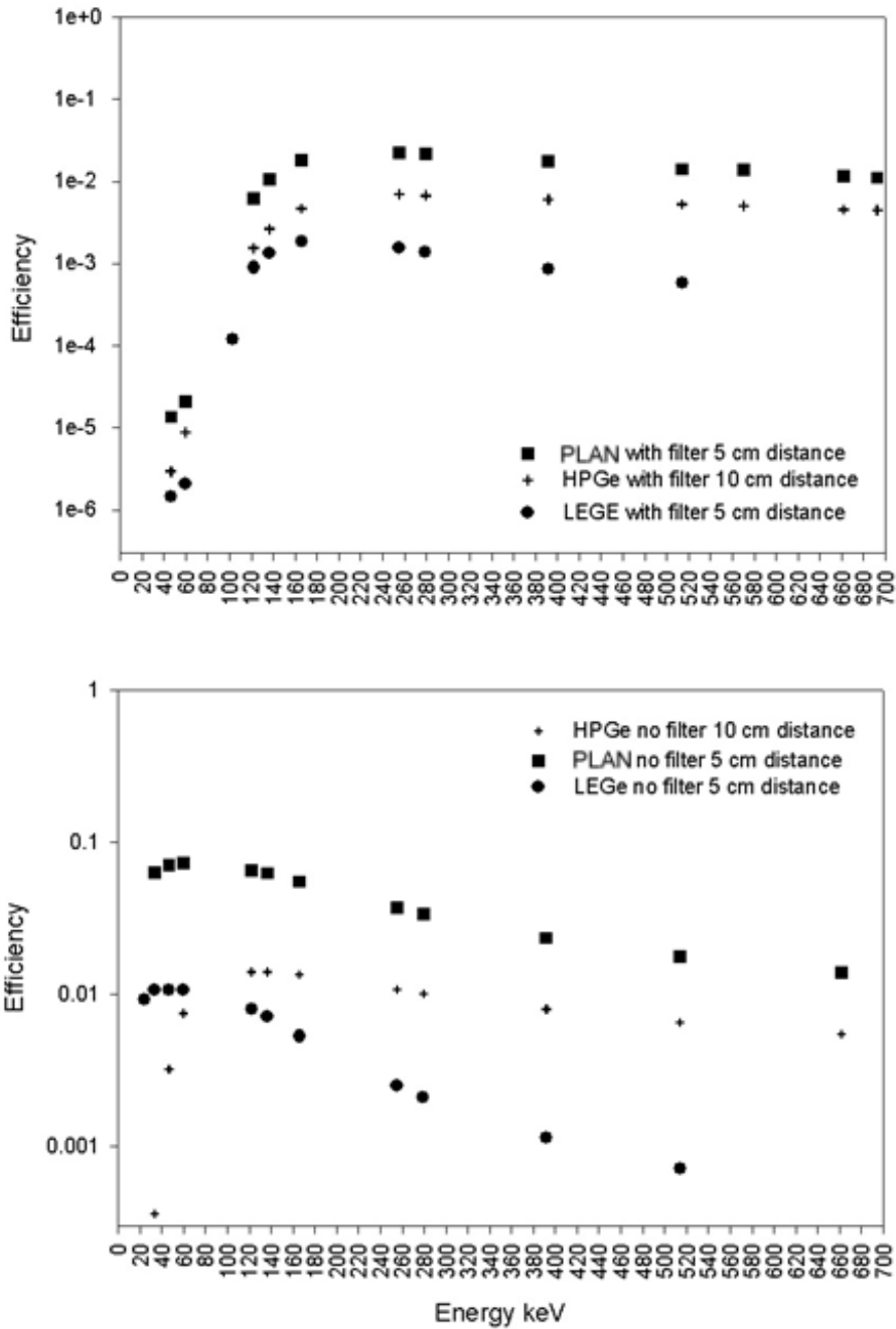
Figure 6. Calibration curves for the three semi-conductor detectors both with and without filters.
