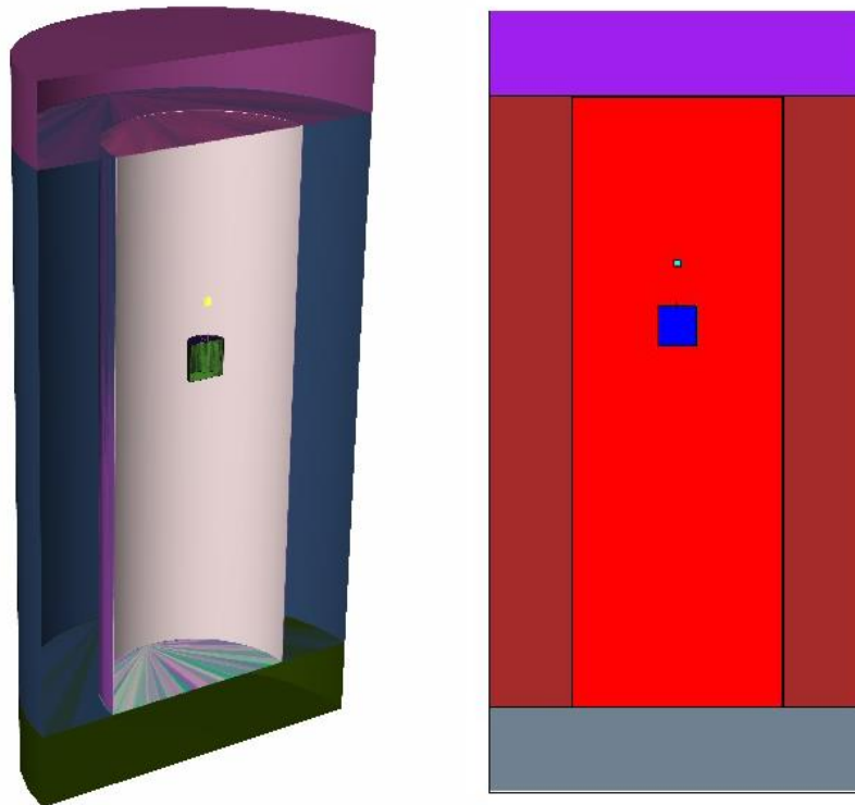
Figure 5. Sectional views of the \text{LaBr}_3 detector within its shield.
