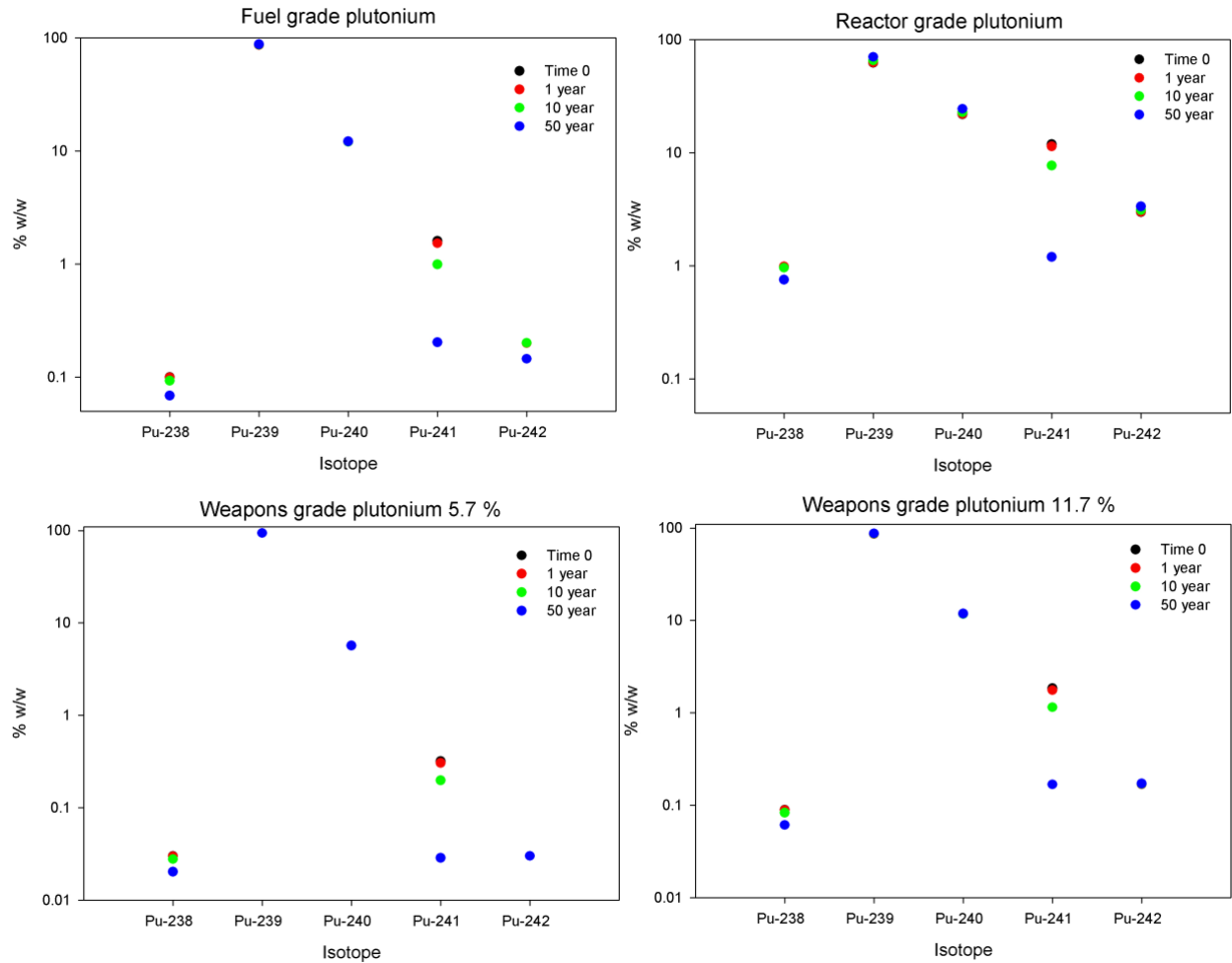
Figure 7. Compositional changes with time for four of the RINFOR materials.
